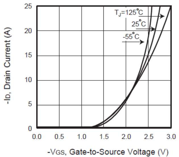
Figure4. Transfer Characteristics
